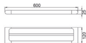
Kara Double Towel Rail 3604-600 (600mm) 3604-800 (800mm)
